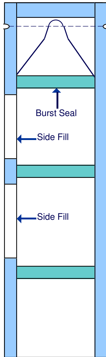
Option 4 with flat die-sealed dispensing tube and triple burst seal side fill
